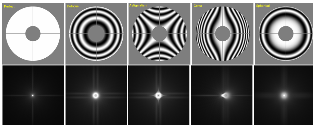
Fig. 1. Real part of the pupil functions and their respective PSFs in the perfect case (left), and in the presence of 1'' (d80) of defocus, astigmatism, coma, and spherical aberrations. The PSFs are free of seeing effects and convolved with a 0.2'' square-shaped pixel footprint.
